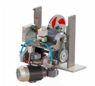
ADR 32 COUNTING HEAD AT 3000 SHEETS/MIN
